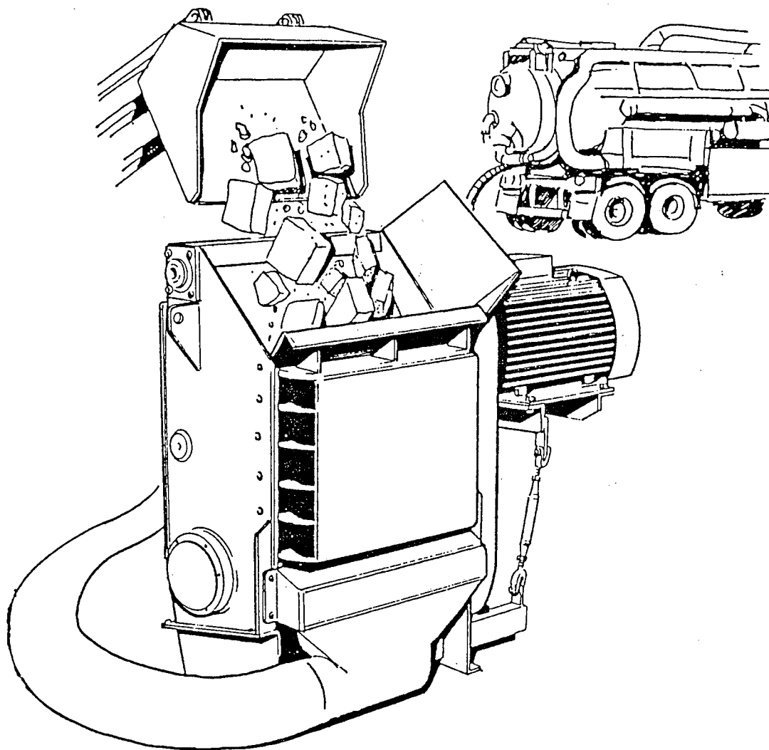
Kross DX 40 under lastning.
